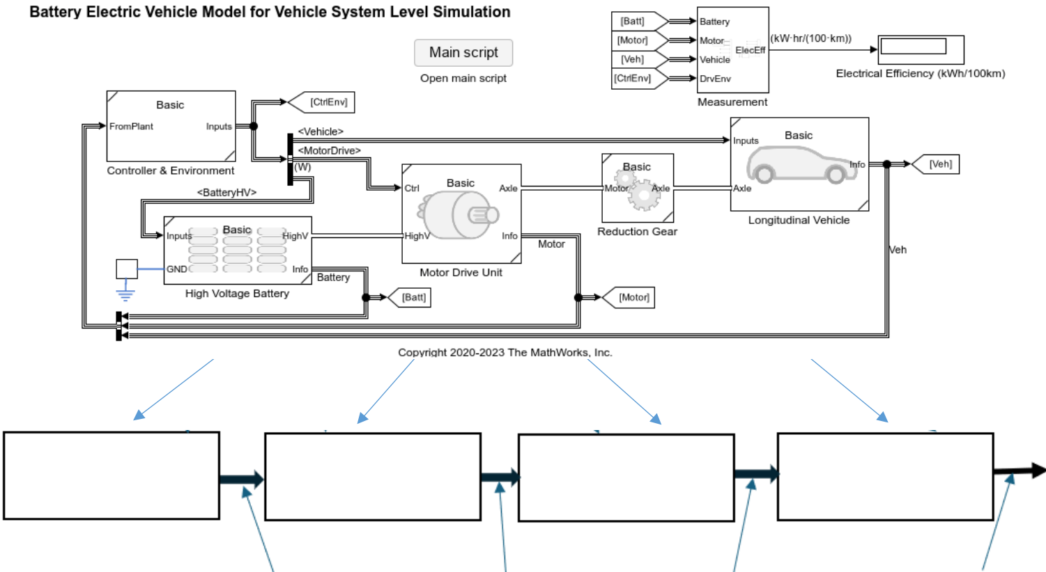
Battery Electric Vehicle Model for Vehicle System Level Simulation
